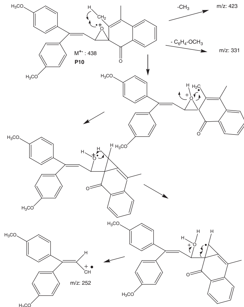
Scheme 5. Proposed fragmentation of P10 following electron impact.
