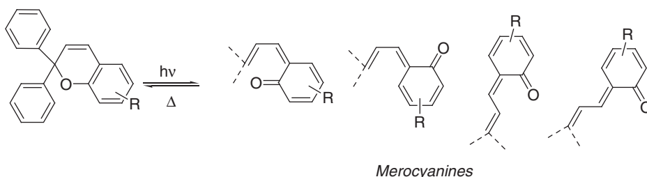
Scheme 1. Reversible photoconversion of chromenes to merocyanines.
