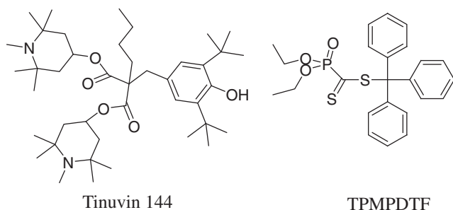
Figure 4. Structures of additives.
