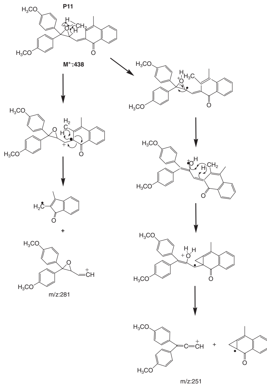
Scheme 6. Proposed fragmentation of P11 following electron impact.
