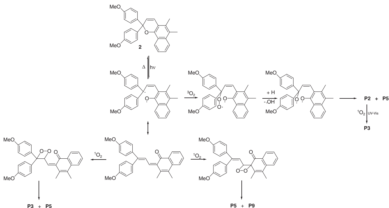
Scheme 4. Possible degradation pathway from compound 2 .
