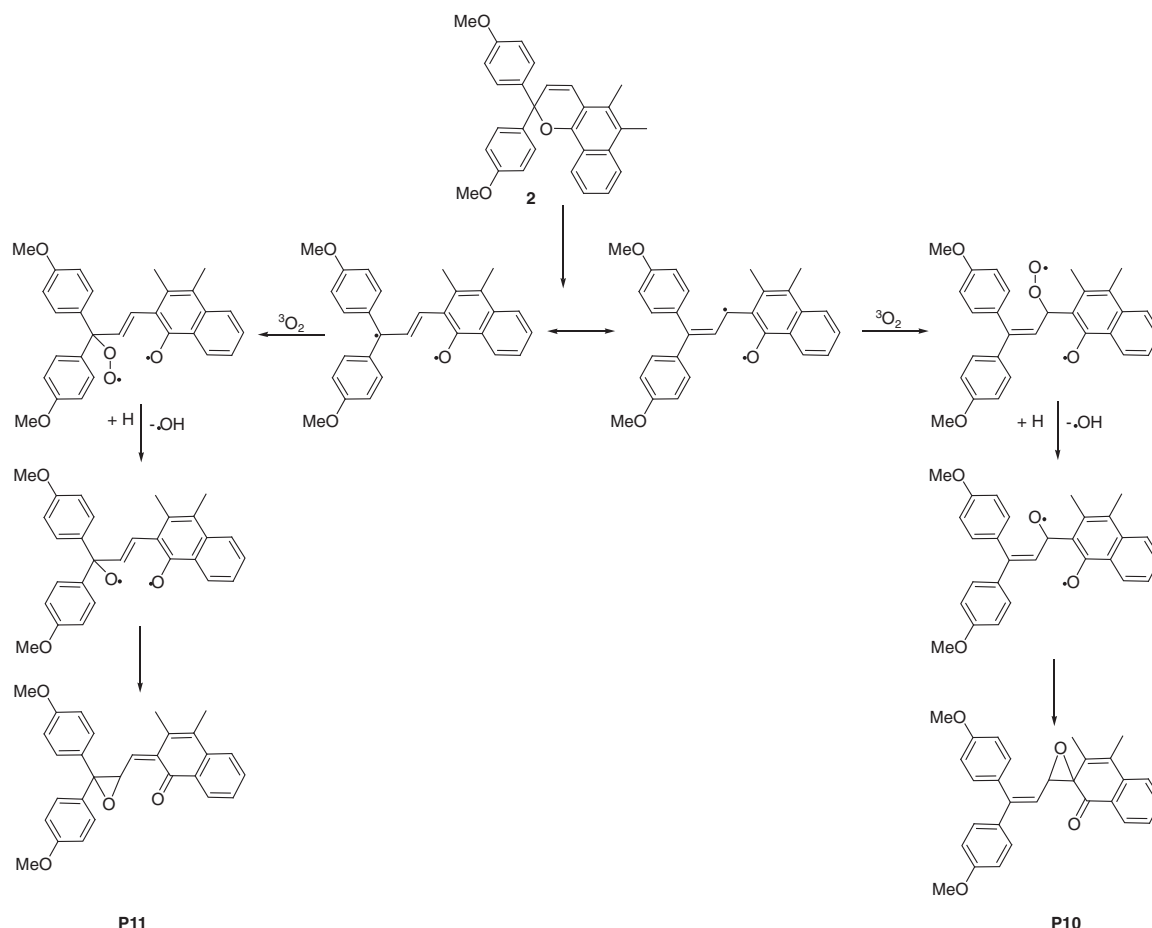
Scheme 2. Speculative mechanisms concerning the formation of epoxides P10 and P11 .
