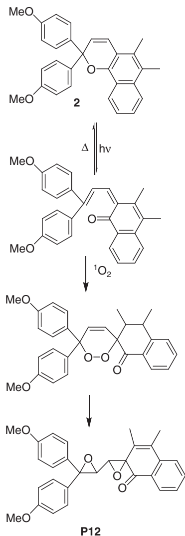
Scheme 3. Speculative mechanisms concerning the formation of P12 .
