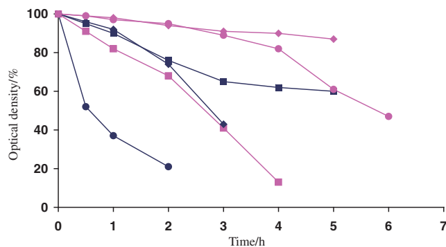
Figure 3. Time profile of the optical density exhibited by compound 2 (●), 3 (◆), and 4 (■) in toluene solution (pink) and in a polyurethane matrix (blue) under stationary irradiation with the light from a 1.5 kW Xenon lamp.
