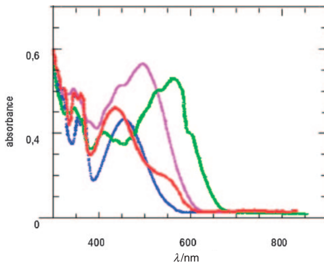
Figure 2. Absorption spectra for the merocyanines from 1 (blue), 2 (green), 3 (red), and 4 (pink) in toluene solution.
